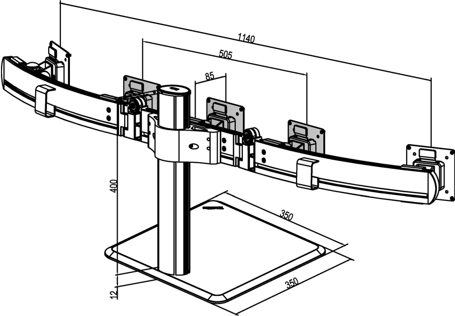
Product Dimensions
